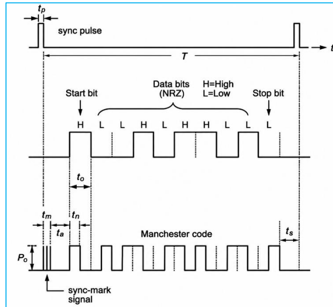
Figure 4. Generation of the Manchester code signal
