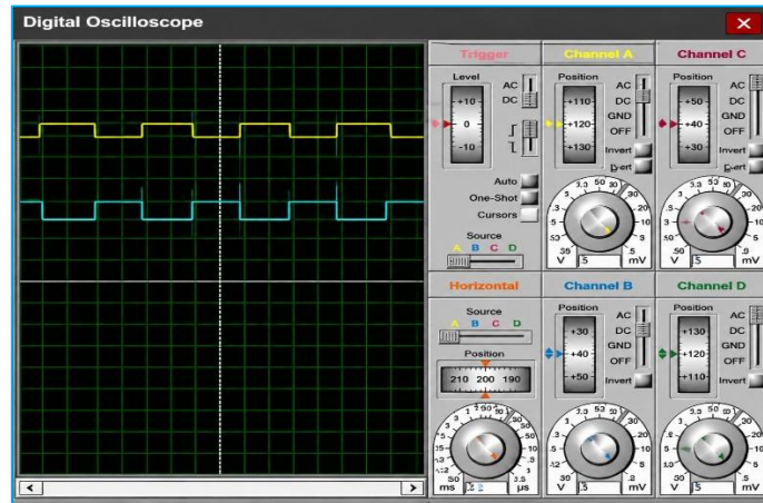
Figure 8. Simulation results of transmitter on digital oscilloscope
