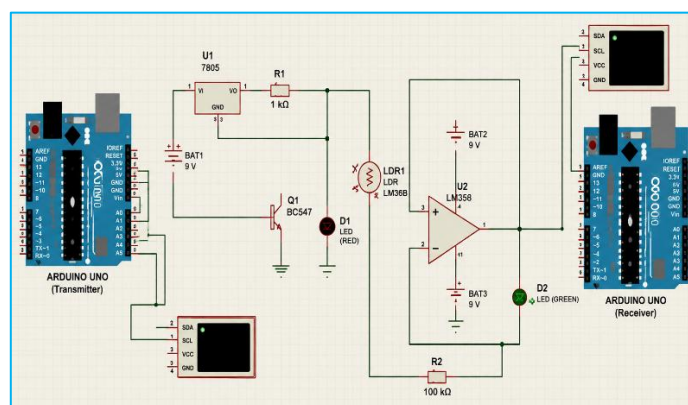
Figure 11. Combine simulation of transmitter and receiver circuit
