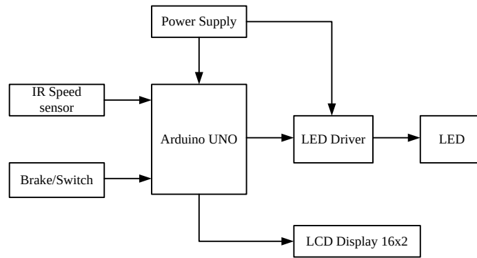
Figure 5. Transmitter section
