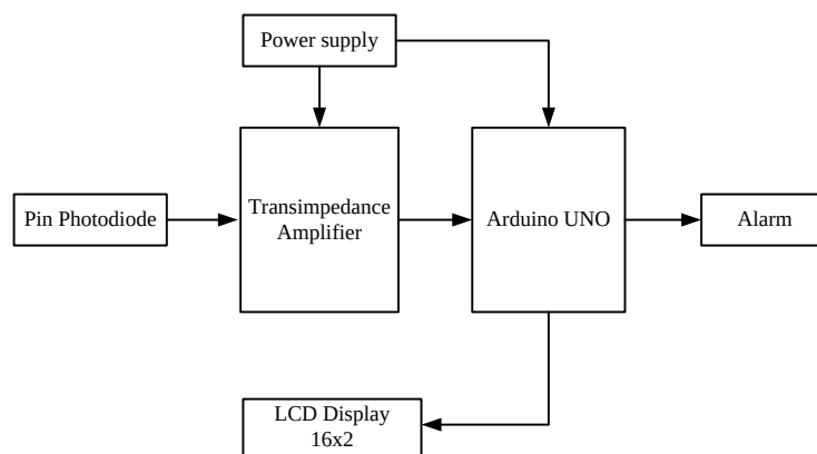
Figure 6. Receiver section
