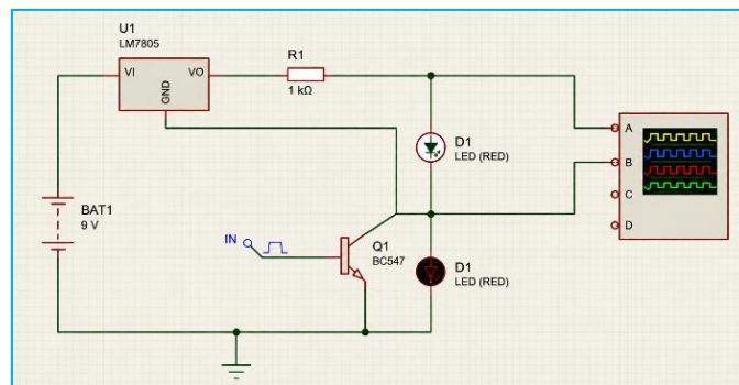
Figure 7. Transmitter side simulation on Proteus 8 software
