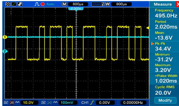
Figure 16. Waveform obtained on DSO for transmitter section
