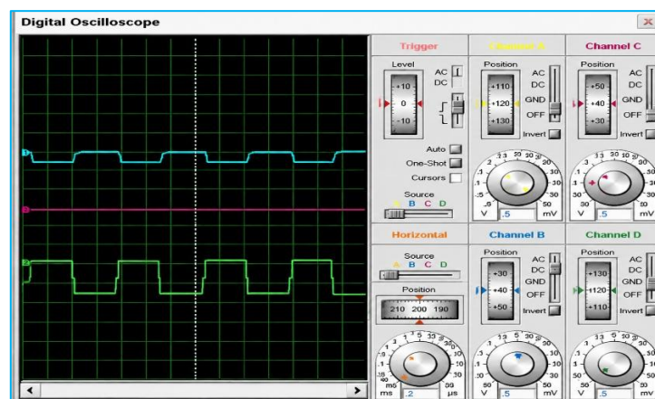
Figure 10. Simulation results of receiver section on digital oscilloscope
