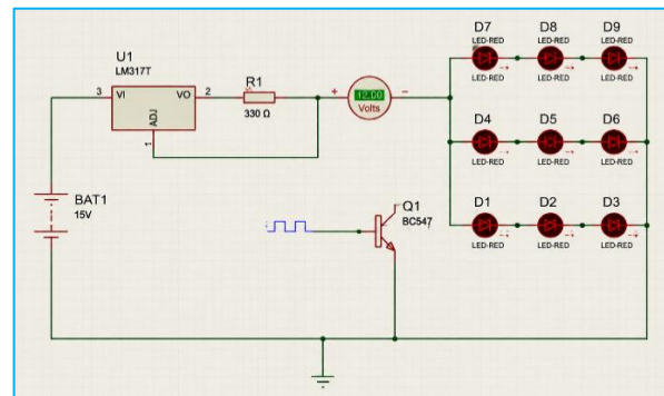
Figure 19. Array of LED's
