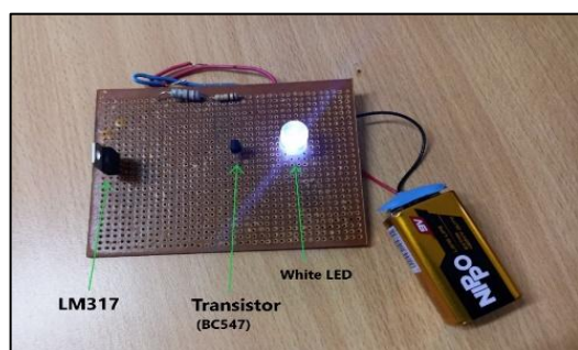
Figure 13. Hardware design of transmitter section
