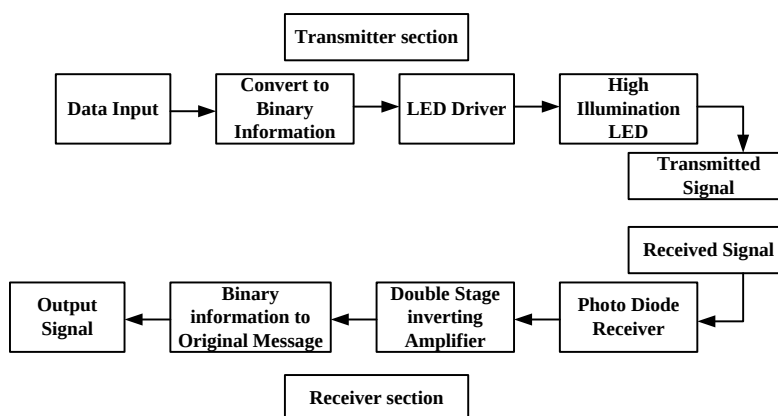
Figure 3. Li-Fi system
