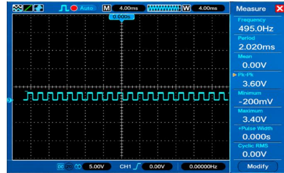
Figure 17. Waveform obtained on DSO for receiver section
