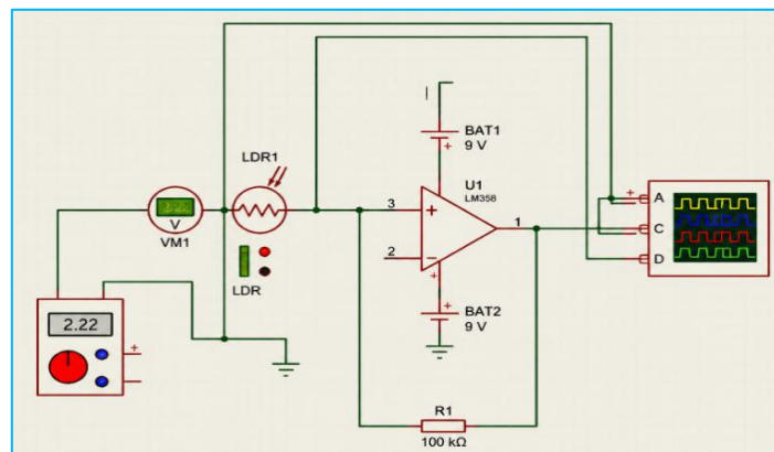
Figure 9. Receiver side simulation on Proteus 8 software
