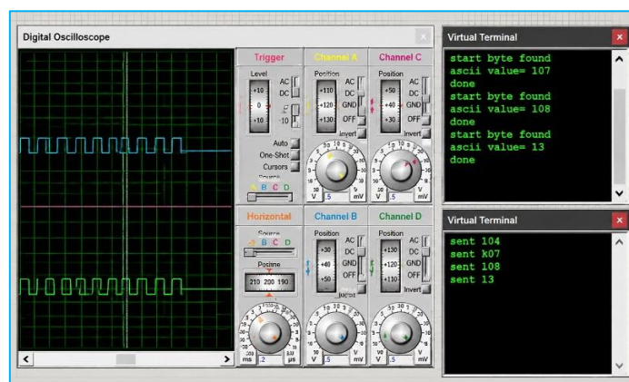
Figure 12. Combine simulation results of transmitter and receiver circuit
