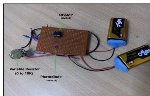
Figure 14. Hardware design of receiver section
