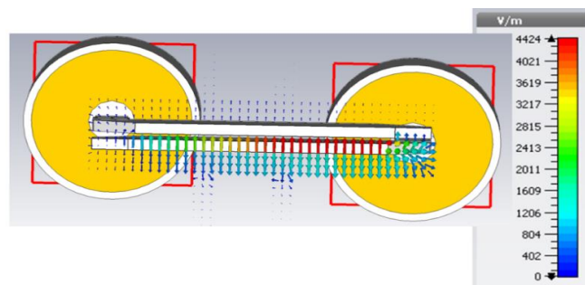
Figure 3. The electric field lines pattern (cross-view). The simulation is performed using a signal of 1 W fed into the output
