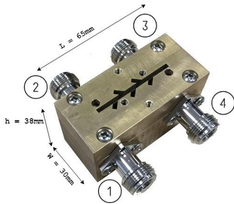
Figure 5. The proposed DGS-coupler is shown
