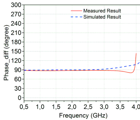
Figure 7. Phase shift among ports
