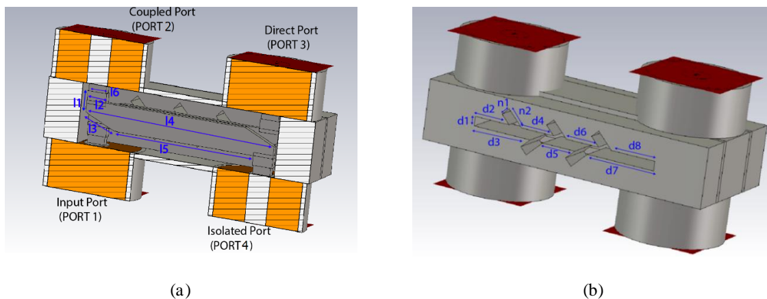
Figure 1.(a) The 3D drawing of the presented quadrature coupler at 2 GHz, (b) The proposed DGS structure introduces the tree-shaped ground slot patterning in the 3D model
