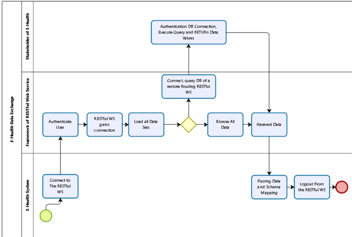
Figure 6. Data exchange of RESTful web service
