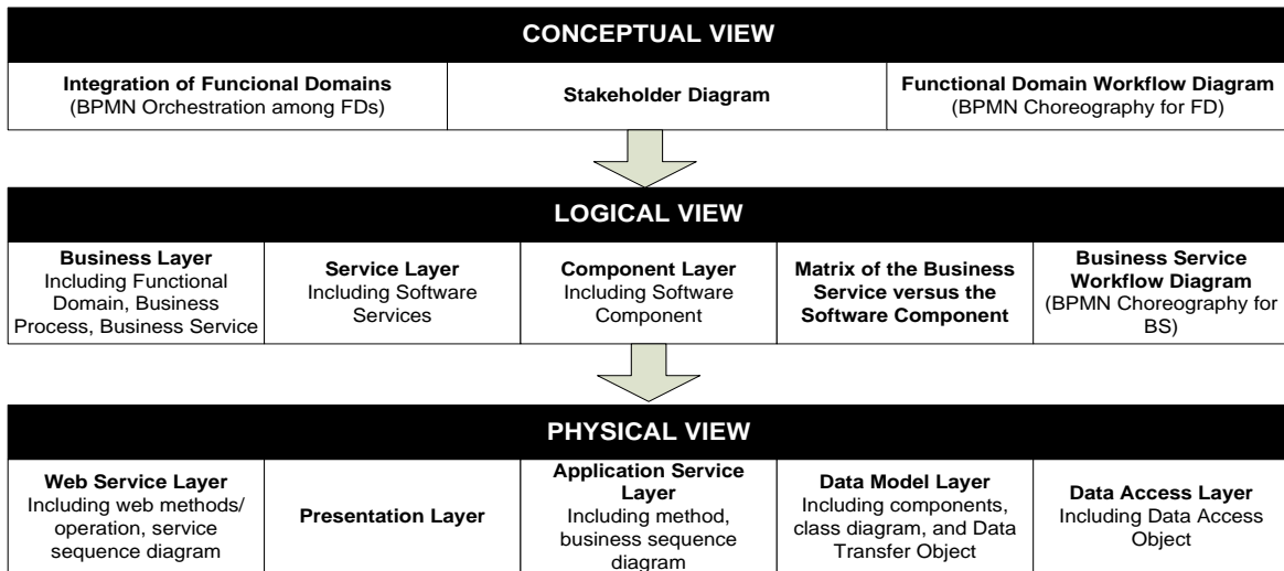
Figure 3. Service portfolio SOAD framework
