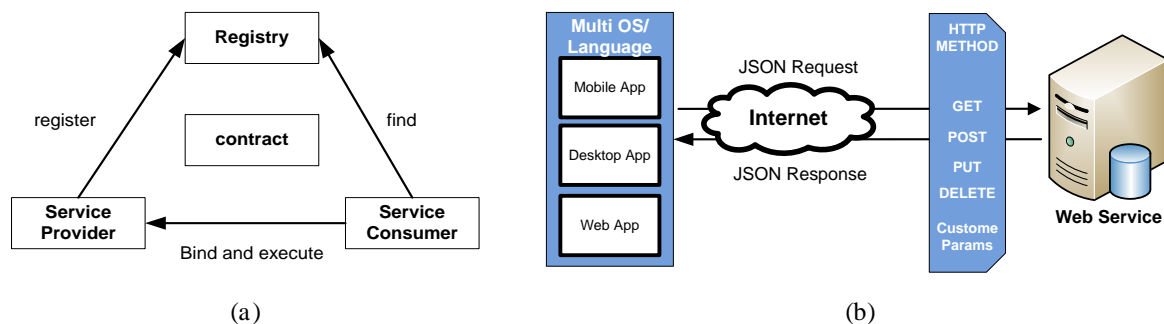
Figure 2. SOAP and REST protocol, (a) SOAP protocol (adapted from [19]), (b) REST protocol (adapted from [3])
