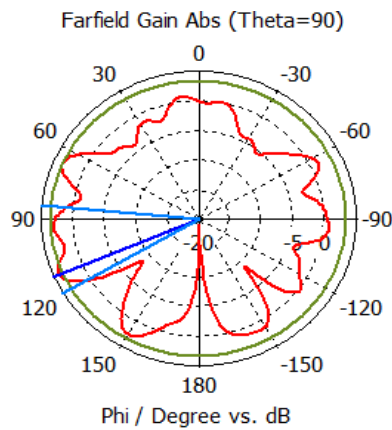
Figure 9. The radiation patterns of proposed filter antenna in E-plane &amp; H-plane at f=5.5 GHz
