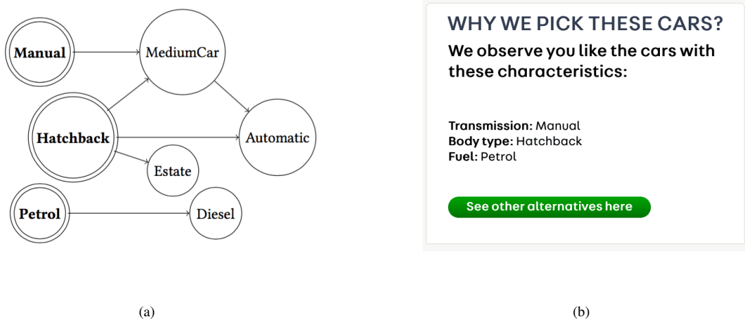
Figure 2. Explanation of the Recommendation System, (a) Directed graph of user preferences, (b) Recommendation explanation
