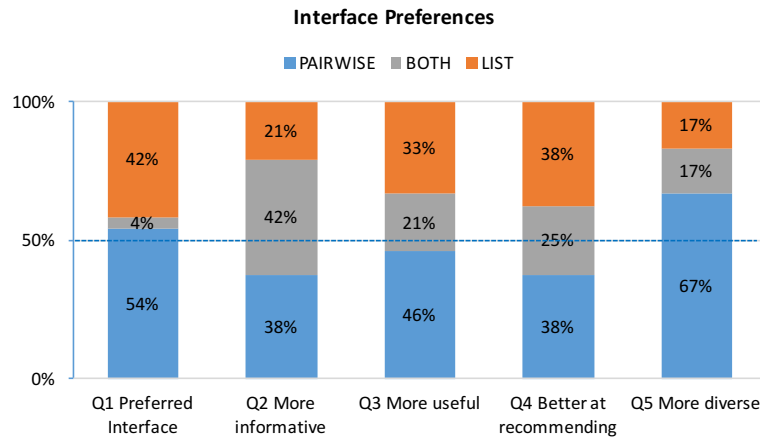
Figure 7. Interface preferences questionnaire results
