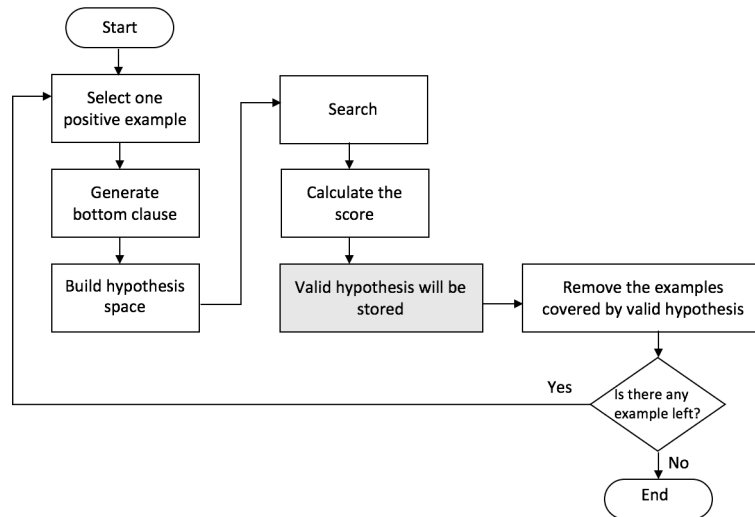
Figure 1. APARELL Learning Step (grayed box shows the process where the valid rules produced as the output of the algorithm)
