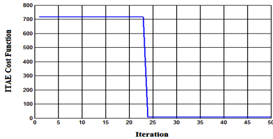
Figure 4. ITAE function for the backstepping controller according to SSA tuning
