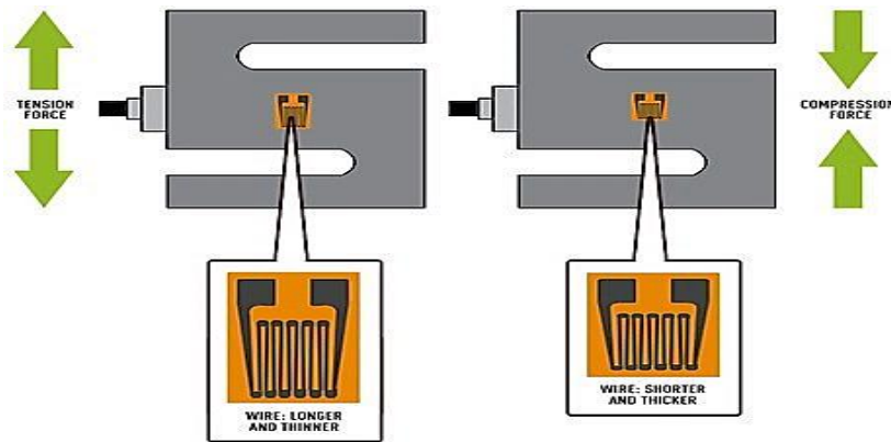
Figure 5. Strain gauge
