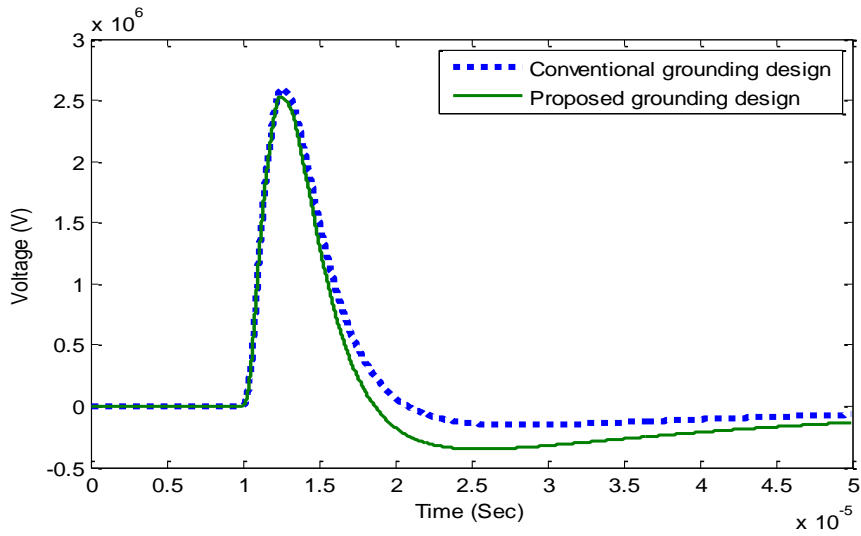
Figure 9. Tower top voltage under only 51kA 8/20µs
