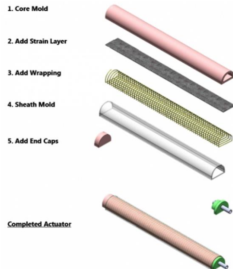
Figure 2. Fiber-reinforced components
