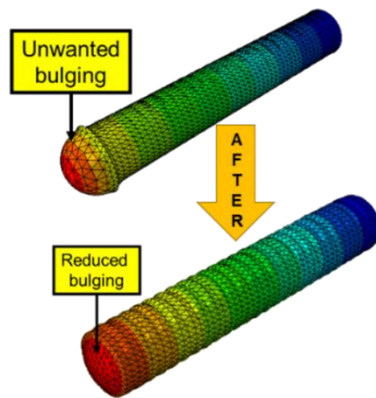
Figure 16. Result after optimizing R10 design
