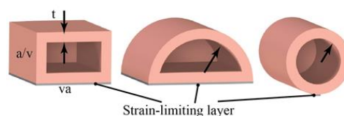
Figure 7. Common cross-sectional shapes in soft actuator designs; circular, rectangular, and semi-circular
