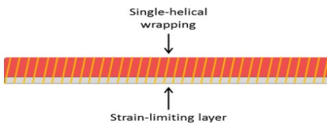
Figure 5. Fiber-reinforced design for twisting and bending motions
