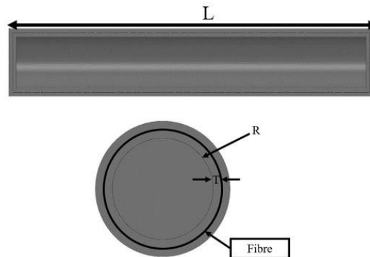
Figure 10. Parameters of fiber-reinforced design
