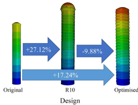
Figure 18. Comparison of improvements in the extension of original, R10, and optimized design
