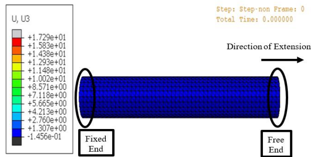
Figure 14. Fiber-reinforced soft actuator simulation
