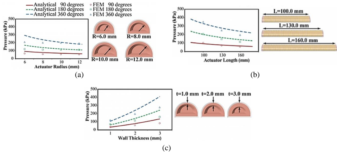
Figure 8. Analysis of optimizing parameters for linear fiber-reinforced soft actuators of; (a) actuator radius, (b) actuator length, and (c) actuator walls thickness
