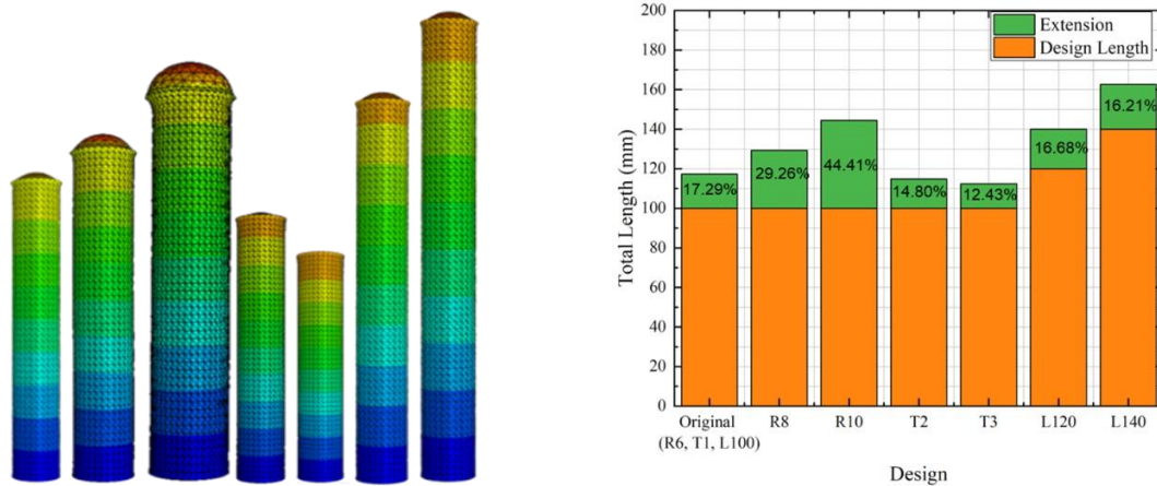
Figure 15. Results of simulation vs graph of total length for each design
