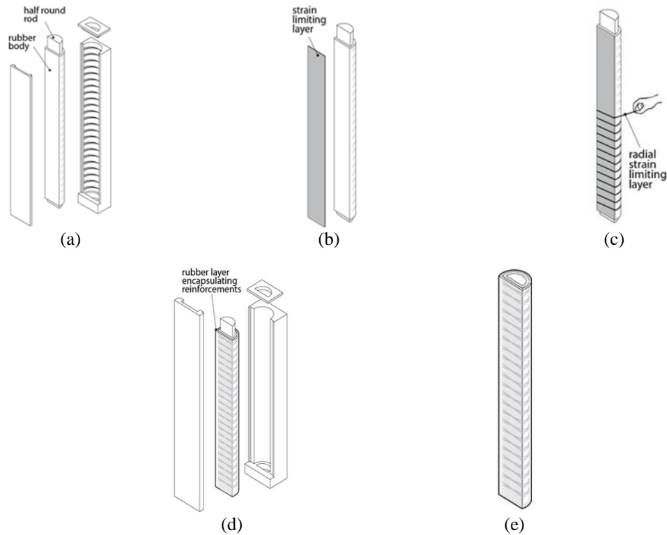
Figure 9. Fiber-reinforced molds and fabrication process of; (a) semi-circular rod mold, (b) assembly of the strain-limiting layers, (c) the fiber reinforcements wrapped around the actuator, (d) the outer silicone sheath, molded over the fibers, and (e) completed linear fiber-reinforced soft actuator [31]
