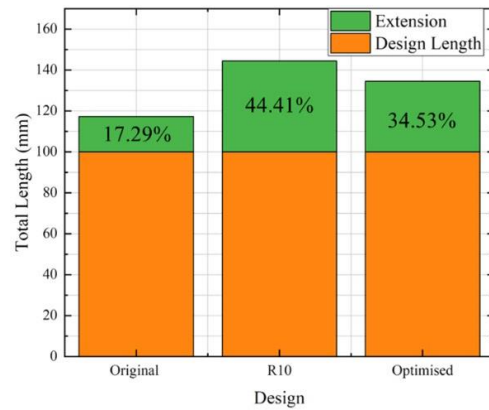
Figure 17. Graph of total length for original, R10, and optimized design
