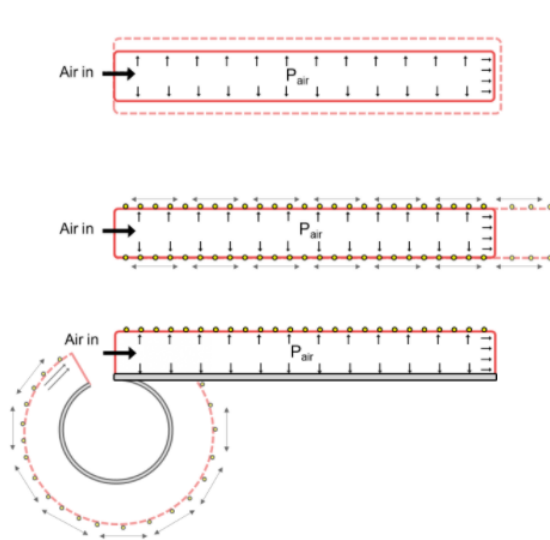
Figure 1. Fiber-reinforced design principal operation when pressurized
